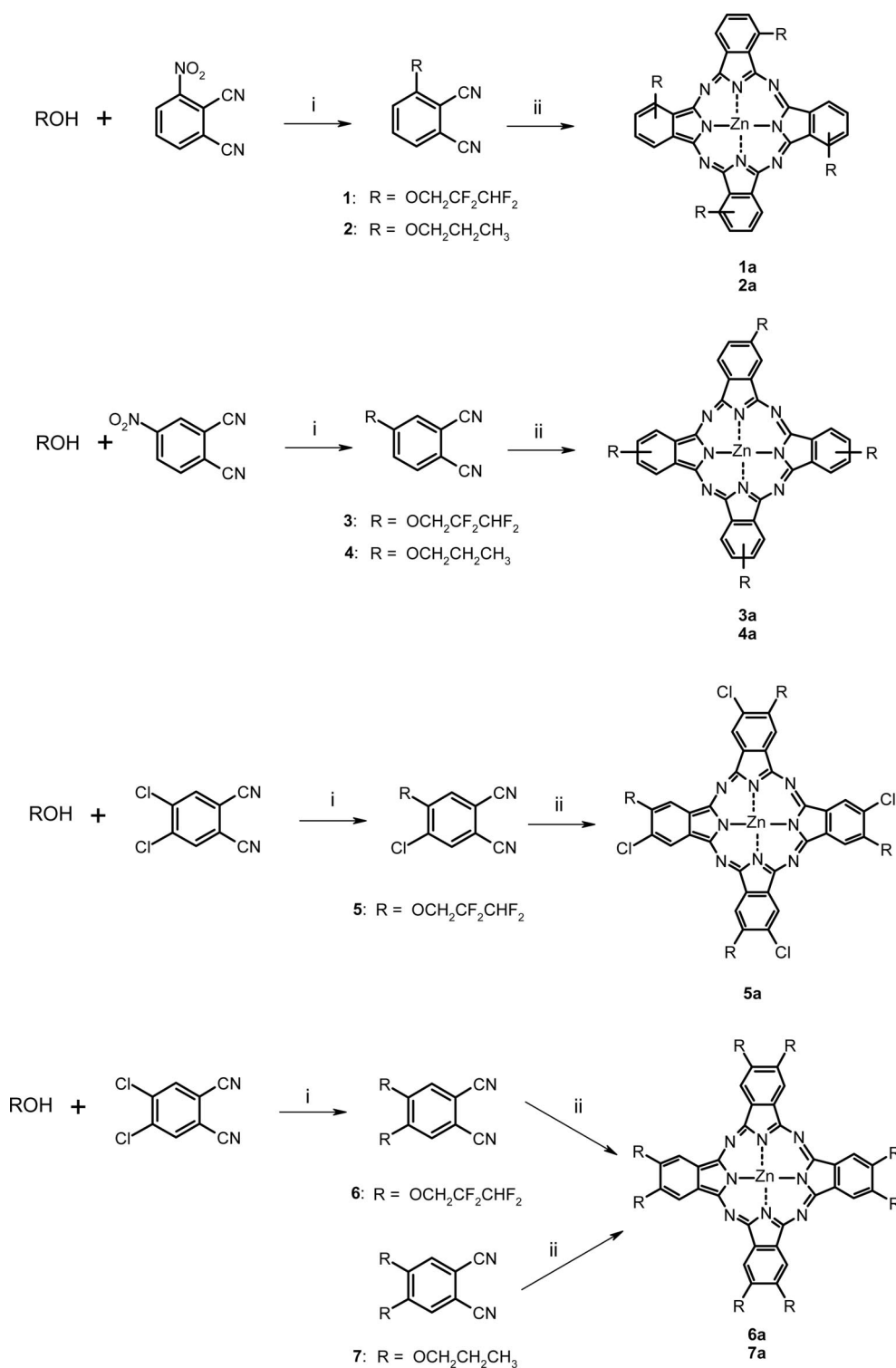
Scheme 1. Chemical pathway used to synthesize the tetra- ( 1a , 2a , 3a , 5a ) and octasubstituted ( 6a , 7a ) phthalocyanine derivatives; (i) K_2CO_3 , DMSO, room temperature, 24 h; (ii) n -amyl alcohol, DBU, zinc acetate, reflux.
