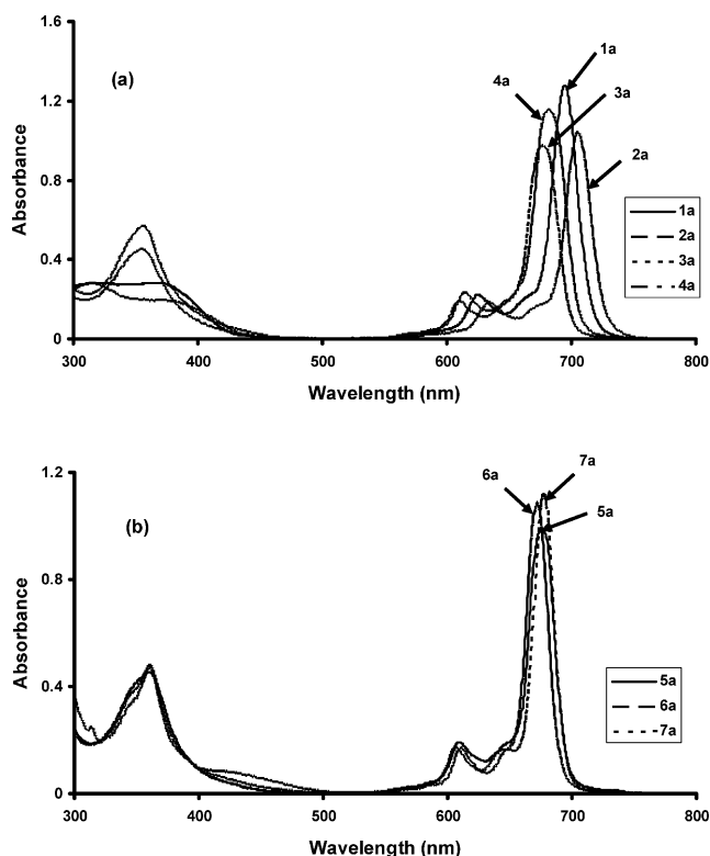
Figure 2. Absorption spectra of (a) tetrasubstituted ( 1a , 2a , 3a and 4a ) and (b) octasubstituted ( 5a , 6a and 7a ) phthalocyanines in DMSO. Concentration: approximately 4 \times 10^{-6} \text{ mol dm}^{-3} .
