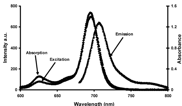
Figure 6. Absorption, excitation and emission spectra for compound 1a in DMSO. Excitation wavelength = 670 nm.
