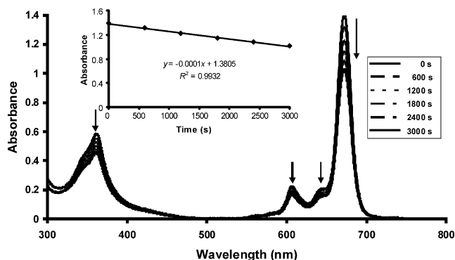
Figure 8. The photodegradation of compound 6a in DMSO showing the disappearance of the Q band at 10 min intervals. Inset: plot of absorbance versus time.
