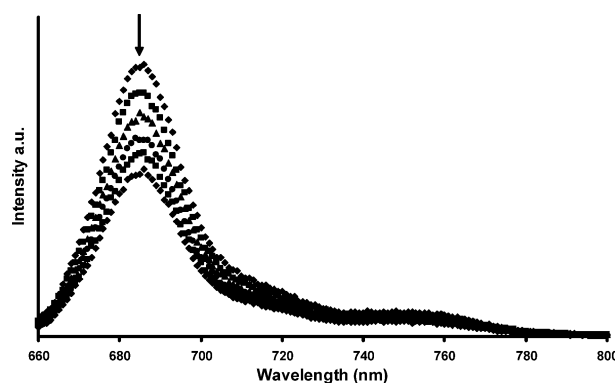
Figure 9. Fluorescence emission spectral changes of 5a ( 1.00 \times 10^{-5} \text{ mol dm}^{-3} ) upon addition of different concentrations of BQ in DMSO. [BQ] = 0, 0.008, 0.016, 0.024, 0.032, 0.040 \text{mol dm}^{-3} .
