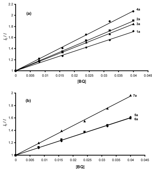
Figure 10. Stern-Volmer plots for benzoquinone (BQ) quenching of (a) 1a , 2a , 3a , 4a and (b) 5a , 6a , 7a . [MPc] = approximately 1.00 \times 10^{-5} \text{ mol dm}^{-3} in DMSO. [BQ] = 0, 0.008, 0.016, 0.024, 0.032, 0.040 \text{mol dm}^{-3} .
