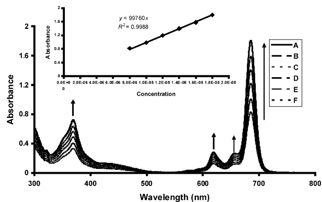
Figure 5. Aggregation behaviour of 7a in DMSO at different concentrations: 18 \times 10^{-6} (A), 16 \times 10^{-6} (B), 14 \times 10^{-6} (C), 12 \times 10^{-6} (D), 10 \times 10^{-6} (E), 8 \times 10^{-6} (F) \text{mol dm}^{-3} . Inset: plot of absorbance versus concentration.
