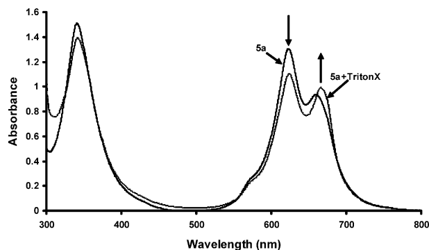
Figure 4. Absorption spectral changes for complex 5a observed upon addition of Triton X-100 in methanol.
