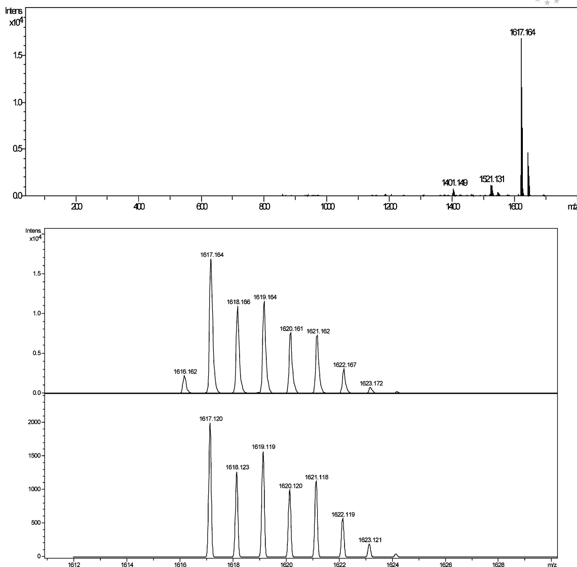
Figure 1. The mass spectrum of compound 6a .
