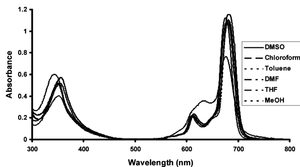
Figure 3. Absorption spectra of 4a in different solvents. Concentration: 4.00 \times 10^{-6} \text{ mol dm}^{-3} .
