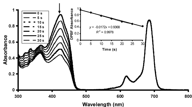
Figure 7. A typical spectrum for the determination of the singlet-oxygen quantum yield. This determination was for compound 3a in DMSO at a concentration of 1 \times 10^{-5} \text{ mol dm}^{-3} . Inset: plot of DPBF absorbance versus time.
